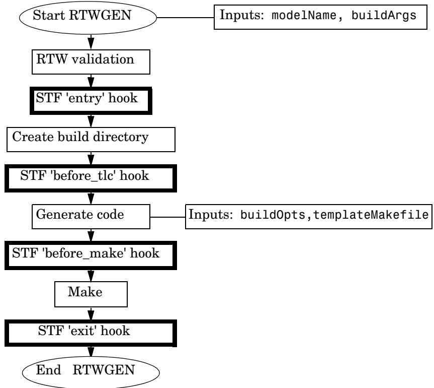
Figure 4-1: Build Process Flowchart (Hook Points Highlighted)
